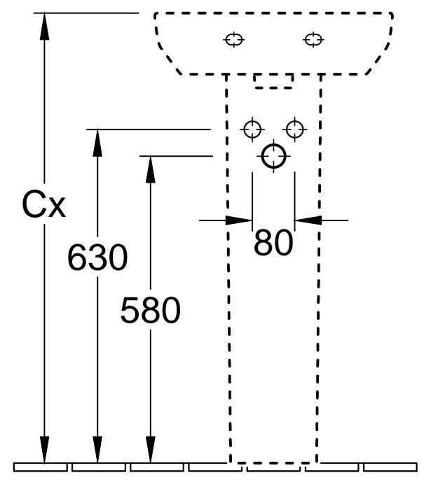
5243 00 Position pedestal to determine Cx
