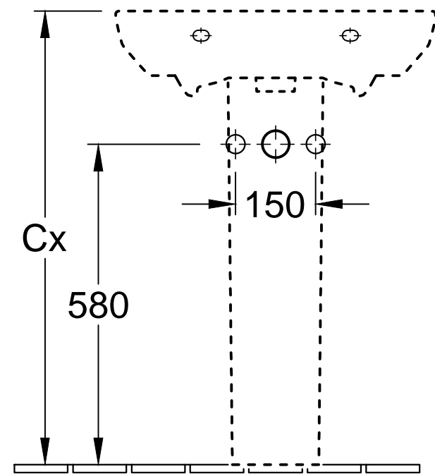
5243 00 Position pedestal to determine Cx
